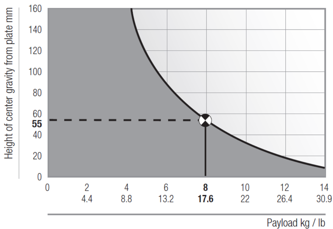
COUNTERBALANCE GRAPH
